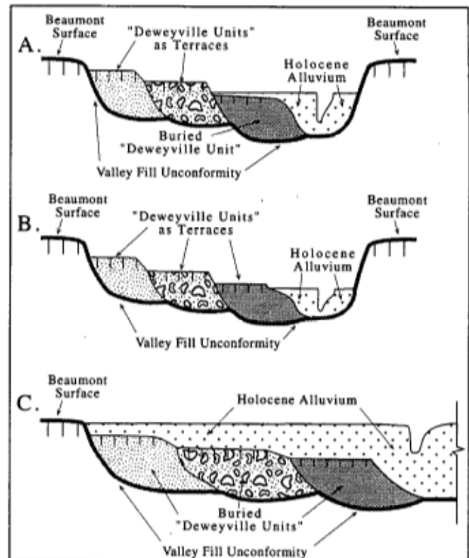
Figure 4. Schematic valley cross-sections contrasting "Deweyville" allostratigraphy" in different geomorphic settings along the Texas Coastal Plain, at similar distances updip from modern highstand shorelines. (a) Low-gradient basin fringe fluvial axis, where high and intermediate Deweyville surfaces remain as terraces, but low Deweyville surfaces occur at the same elevation as modern floodplains, and are veneered by floodplain / delta plain strata. (b) Steep-gradient basin fringe fluvial axis, where low Deweyville surfaces remain as a terrace above modern floodplains until onlapped at modern bay-head deltas. (c) Extrabasinal fluvial axes, where all "Deweyville" surfaces have been onlapped and buried by Holocene strata, and post-Beaumont valleys are nearly filled. Relative scale of valley fill sequences as indicated. "Deweyville" allostratigraphic units are shown occurring on one side of the valley for illustration purposes only.
