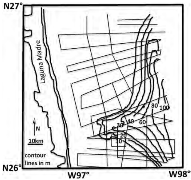
Fig. 13. Structure contour map of Rio Grande incised valley and associated lowstand delta-fan complex.
