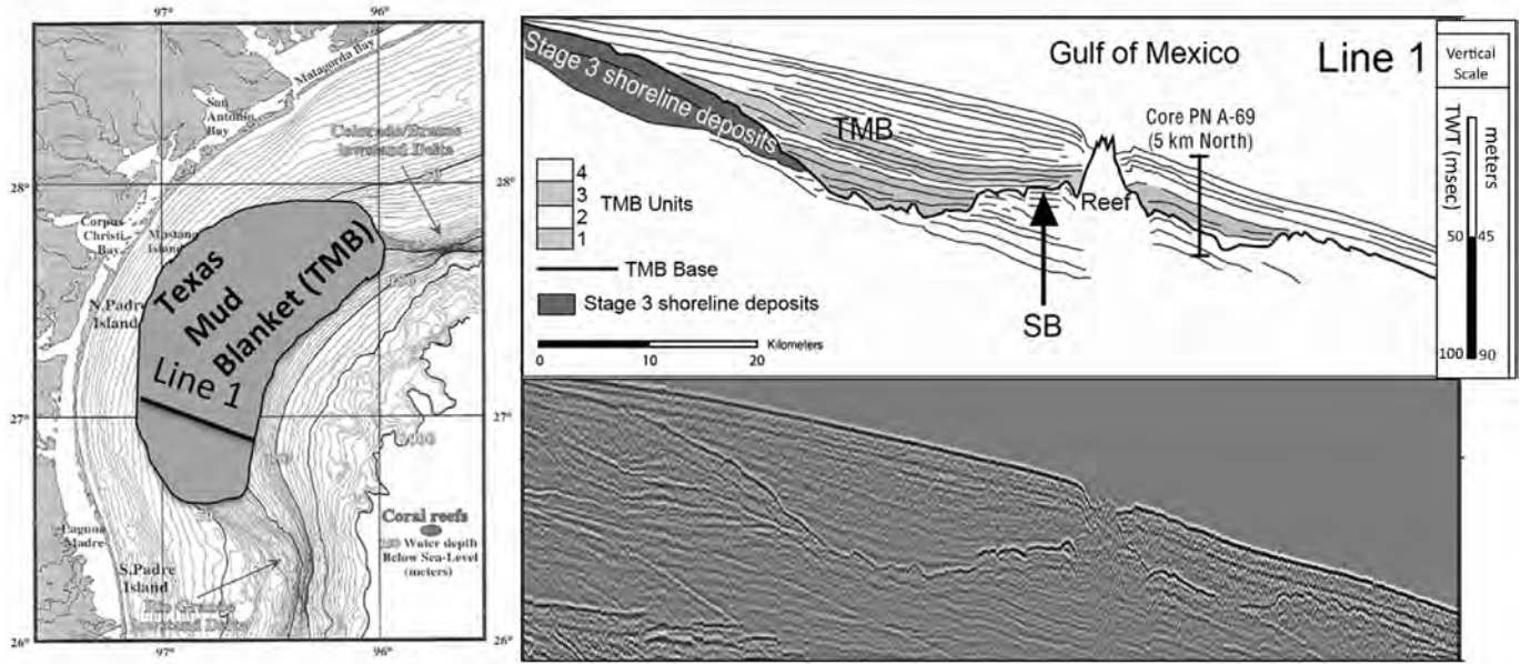
Fig. 29. Interpreted and uninterpreted seismic Line 1 illustrating acoustically laminated character of the Texas Mud Blanket and map showing distribution of the mud blanket (modified from Weight et al., 2011). Also shown is the location of Line 1. Conversion of two-way travel time to meters was done using 1807 m/s and is only valid above sequence boundary.
