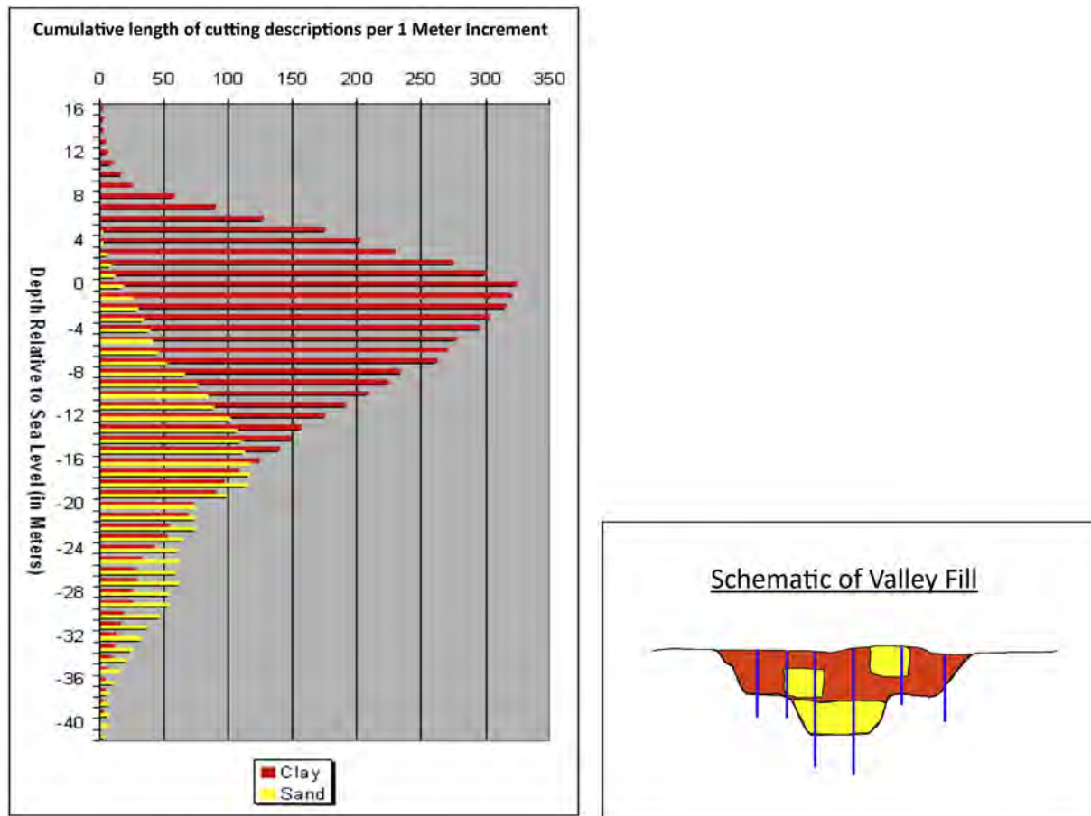
Fig. 25. Vertical distribution of 8800 m of clay and sand descriptions from water wells logged in the lower 60 km of the Brazos Valley. All chosen cutting descriptions are positioned above the inferred Stage 2 sequence boundary, with surface elevations between 0 and 16 m above sea level, depending on distance from coast.
