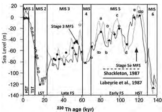
Fig. 2. Composite oxygen isotope records (modified from Labeyrie et al., 1987; Shackleton, 1987; open circles = Bard et al., 1990; closed circles and triangles = Chappell et al., 1996; Anderson et al., 2004) calibrated with U–Th dates on corals used as a proxy sea-level curve for this paper. Also shown are the marine oxygen isotope (MIS) stages. The most poorly constrained portion of the curve is the initial MIS 3 lowstand and highstand, which have uncertainties of up to 30 m.
