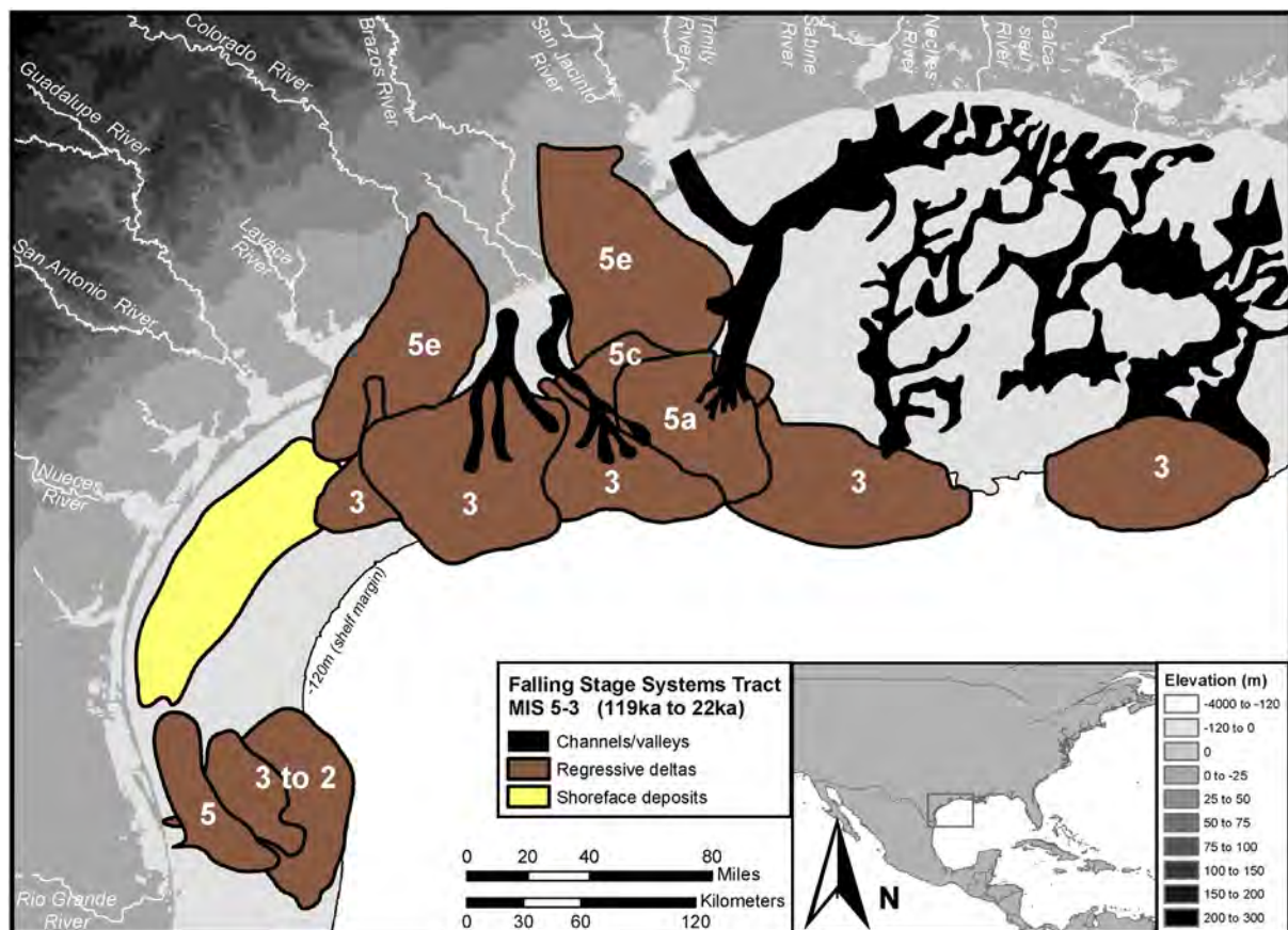
Fig. 9. Paleogeographic map showing major falling-stage depositional systems of the study area (compiled from Suter and Berryhill, 1985; Anderson et al., 2004). Note the repeated cycles of progradation and backstepping exhibited by the Brazos delta.
